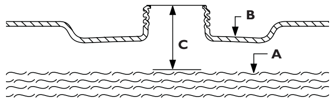
Figure 2 — Fuel Expansion
